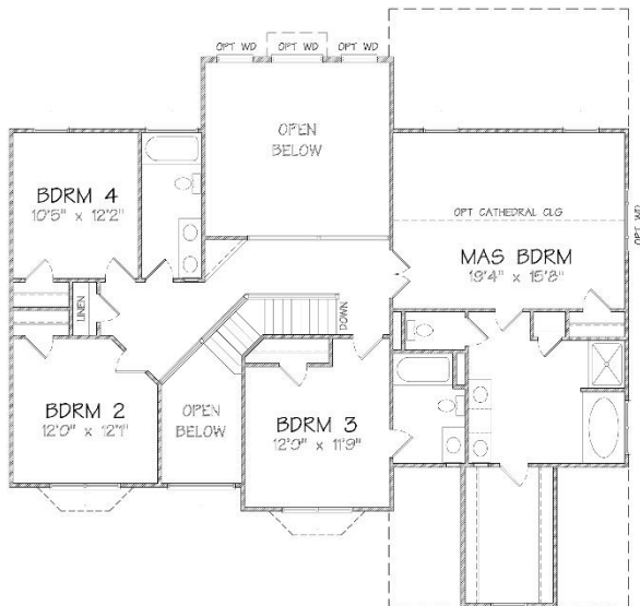
TOP LEVEL
