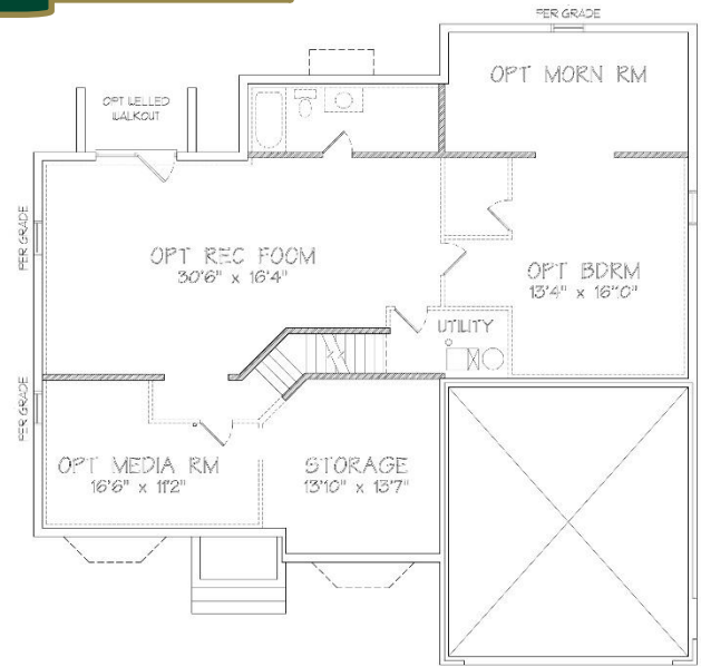
BASEMENT LEVEL
