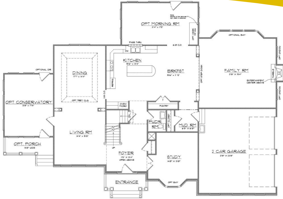
MAIN LEVEL
